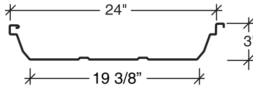
ALLOWABLE UNIFORM LOADS IN POUNDS PER SQUARE FOOT
