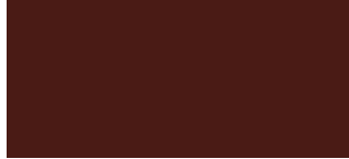
Rustic
