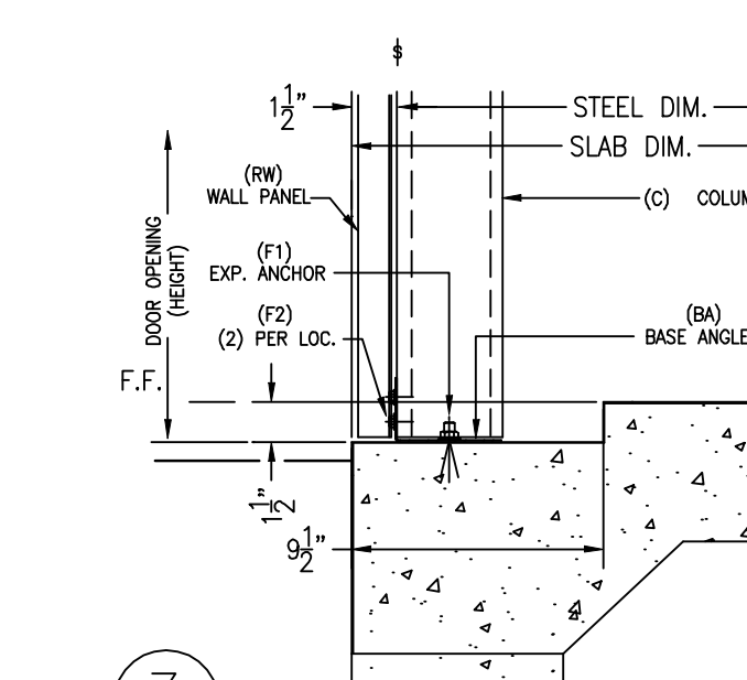
3 SHEETED WALL EDGE BASE
