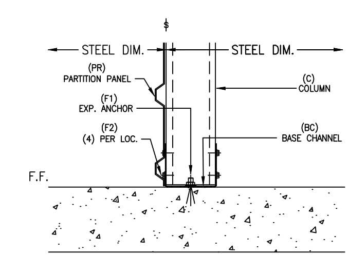
4 FLOOR BASE CHANNEL AT PARTITION WALL
